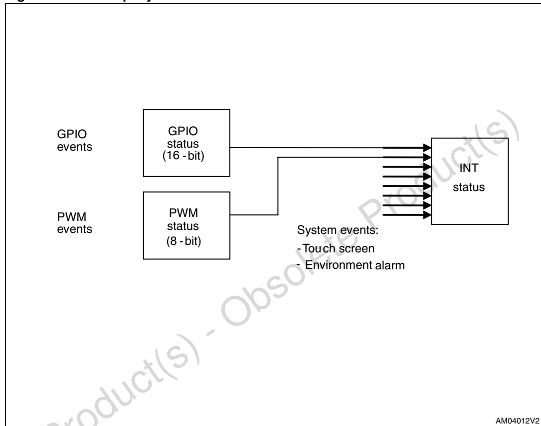
Figure 7. Interrupt system
